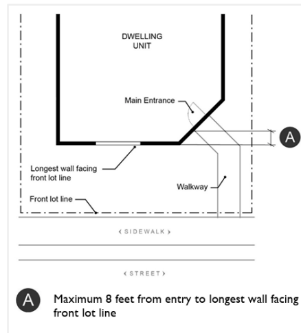
Figure 9.50.0X0.b Main Entrance at 45° Angle from the Street
