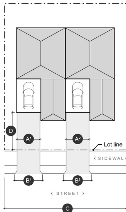
Figure 9.50.0X0.d Width of Garages and Parking Areas
