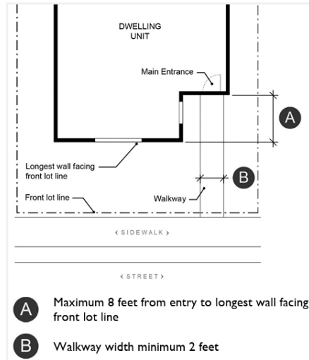
Figure 9.50.0X0.a Main Entrance Facing the street
