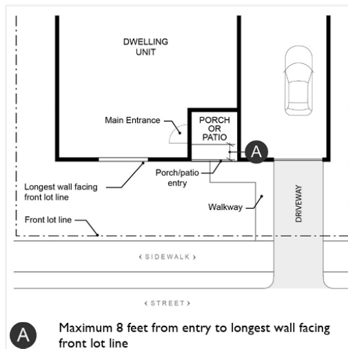
Figure 9.50.0X0.c Main Entrance Opening onto a Porch
